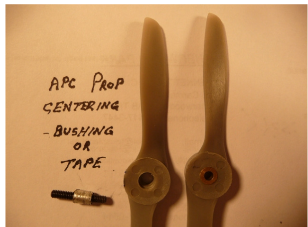
Centering APC props w/ a big prop hole: Use of a bushing, aluminium tape or thin fuel tubing can all be used here.
