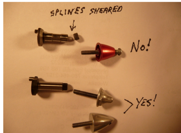
A 5-40 TPI prop stud (screwed ALL the way in) & spinner is used to prevent the Killer Bee/Venom type crankshafts from shearing at the splines.
